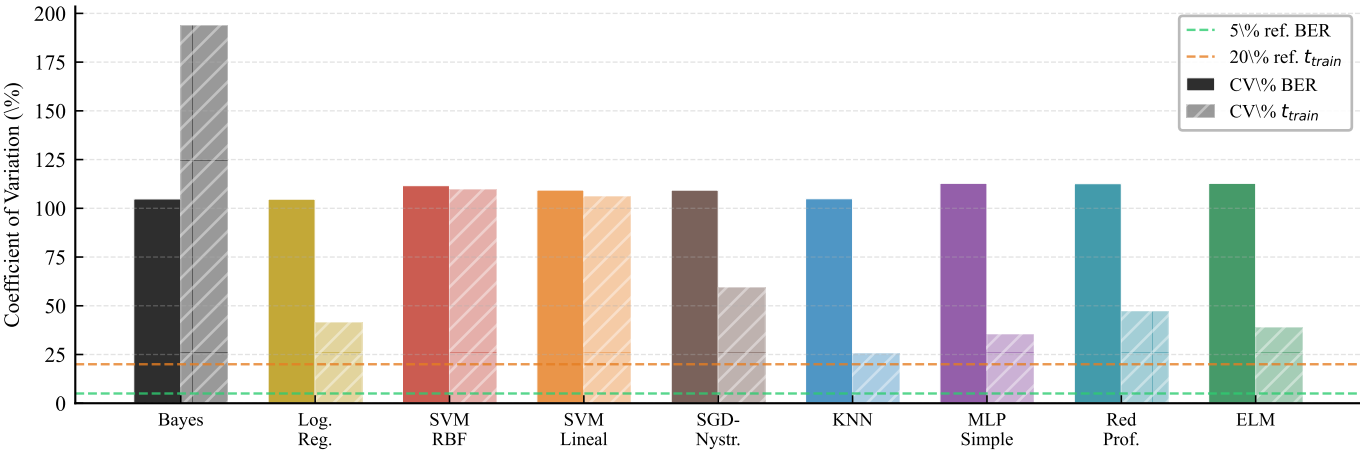
Consistency — CV\% of BER and t_{train} — E_b/N_0 \in [6, 8, 10, 12] dB
